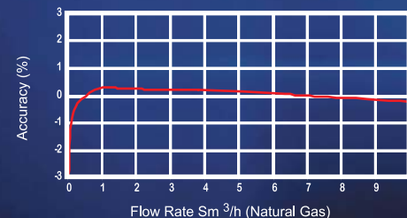
Model 1010 Typical Accuracy Curve
